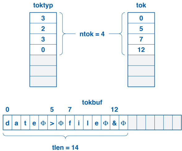
Figure 26.3 Contents of variables tokbuf , toktyp , tok , ntok , and tlen for the input line: date > file &
