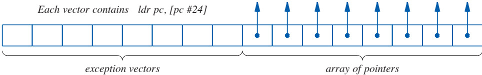
Figure 12.3 ARM exception vectors and an indirect array are contiguous in memory.
